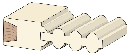
Bevel Profile
